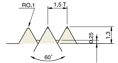
排齒詳圖 Drawing of Serration
