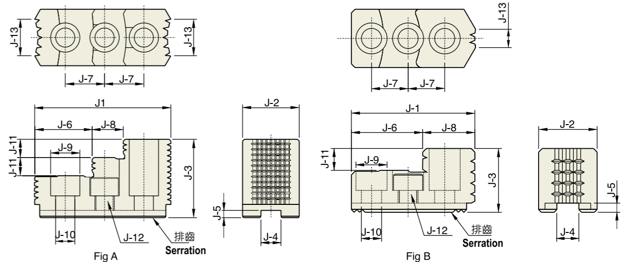
排齒詳圖 Drawing of Serration
